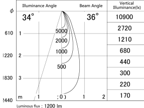
■ Direct Horizontal Illuminance SD379-1035W9030-IK
