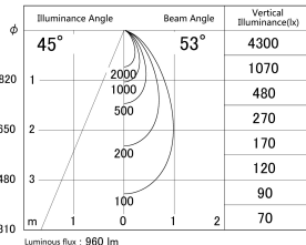
■ Direct Horizontal Illuminance SD379-0955W9040-IK
