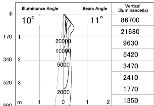
■ Direct Horizontal Illuminance SD381-2015B9030-R
