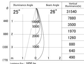
■ Direct Horizontal Illuminance SD386-1525W9027
