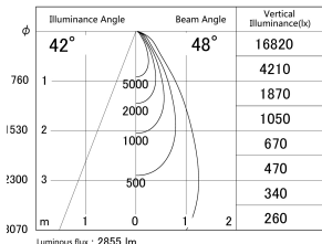
■ Direct Horizontal Illuminance SD386-2550W9027
