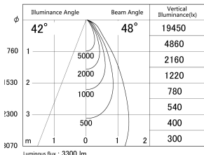
■ Direct Horizontal Illuminance SD386-3050W9027
