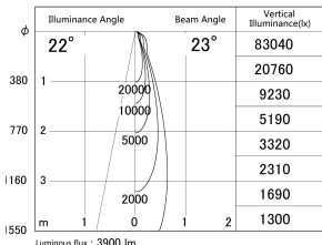
■ Direct Horizontal Illuminance SD386-3525W9027
