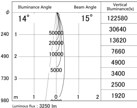
■ Direct Horizontal Illuminance SD386-4015W9027
