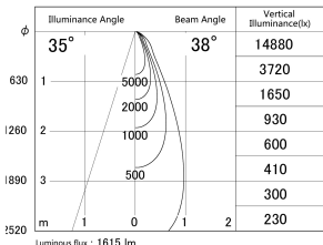
■ Direct Horizontal Illuminance SD386-1535W9030
