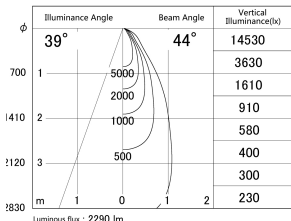
■ Direct Horizontal Illuminance SD386-2050W9030
