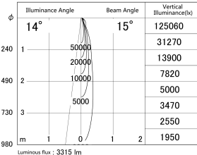
■ Direct Horizontal Illuminance SD386-4015W9030
