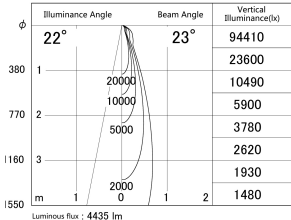
■ Direct Horizontal Illuminance SD386-4025W9030
