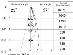
■ Direct Horizontal Illuminance SD386-1025W9035
