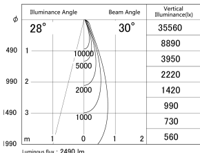
■ Direct Horizontal Illuminance SD386-2035W9035
