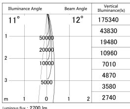
■ Direct Horizontal Illuminance SD386-3015W9035
