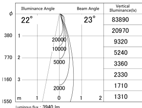
■ Direct Horizontal Illuminance SD386-3525W9035
