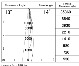
■ Direct Horizontal Illuminance SD386-1015W9040
