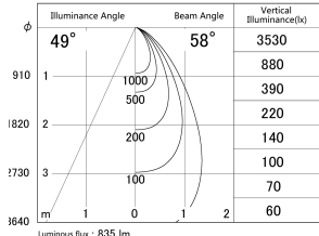
■ Direct Horizontal Illuminance SD386-1050W9040
