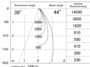
■ Direct Horizontal Illuminance SD386-2050W9040
