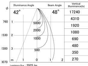
■ Direct Horizontal Illuminance SD386-2550W9040
