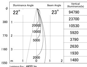
■ Direct Horizontal Illuminance SD386-4025W9040
