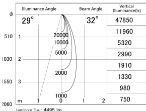
■ Direct Horizontal Illuminance SD386-4035W9040
