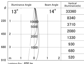
■ Direct Horizontal Illuminance SD386-1015B9027
