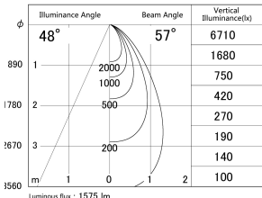
■ Direct Horizontal Illuminance SD386-1550B9027
