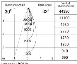
■ Direct Horizontal Illuminance SD386-3035B9027
