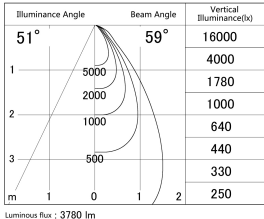
Direct Horizontal Illuminance SD386-3550B9027
