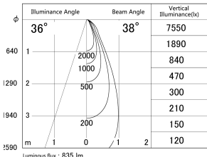
■ Direct Horizontal Illuminance SD386-1035B9030
