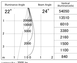
Direct Horizontal Illuminance SD386-2025B9030
