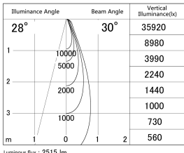
Direct Horizontal Illuminance SD386-2035B9030
