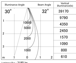
■ Direct Horizontal Illuminance SD386-2535B9030
