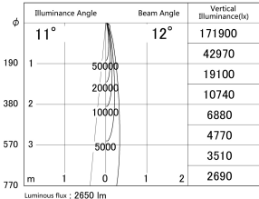
■ Direct Horizontal Illuminance SD386-3015B9030
