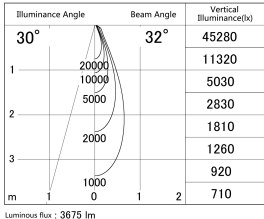
Direct Horizontal Illuminance SD386-3035B9030
