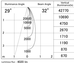
Direct Horizontal Illuminance SD386-3535B9030
