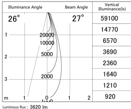
■ Direct Horizontal Illuminance SD386-3025B9035
