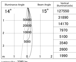
■ Direct Horizontal Illuminance SD386-4015B9035
