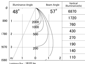
■ Direct Horizontal Illuminance SD386-1550B9040
