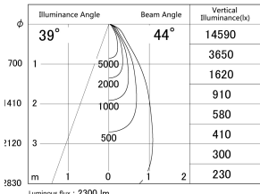
Direct Horizontal Illuminance SD386-2050B9040
