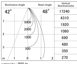
■ Direct Horizontal Illuminance SD386-2550B9040
