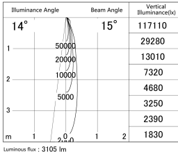
■ Direct Horizontal Illuminance SD386-3515B9040
