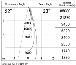
Direct Horizontal Illuminance SD386-3525B9040
