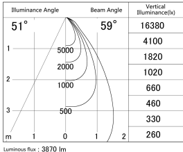
■ Direct Horizontal Illuminance SD386-3550B9040
