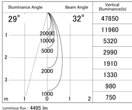
Direct Horizontal Illuminance SD386-4035B9040
