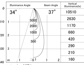
■ Direct Horizontal Illuminance DD161-1035B9027
