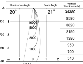
■ Direct Horizontal Illuminance DD161-1520B9027
