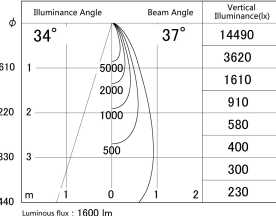
■ Direct Horizontal Illuminance DD161-1535B9027
