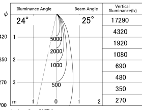
■ Direct Horizontal Illuminance DD161-1025B9030
