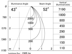
■ Direct Horizontal Illuminance DD161-1550B9030
