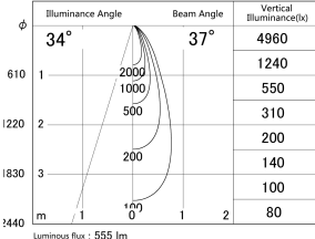
■ Direct Horizontal Illuminance DD161-0535B9035
