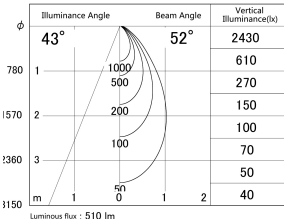
■ Direct Horizontal Illuminance DD161-0550B9035
