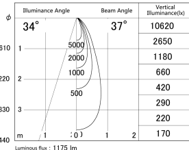
■ Direct Horizontal Illuminance DD161-1035B9035
